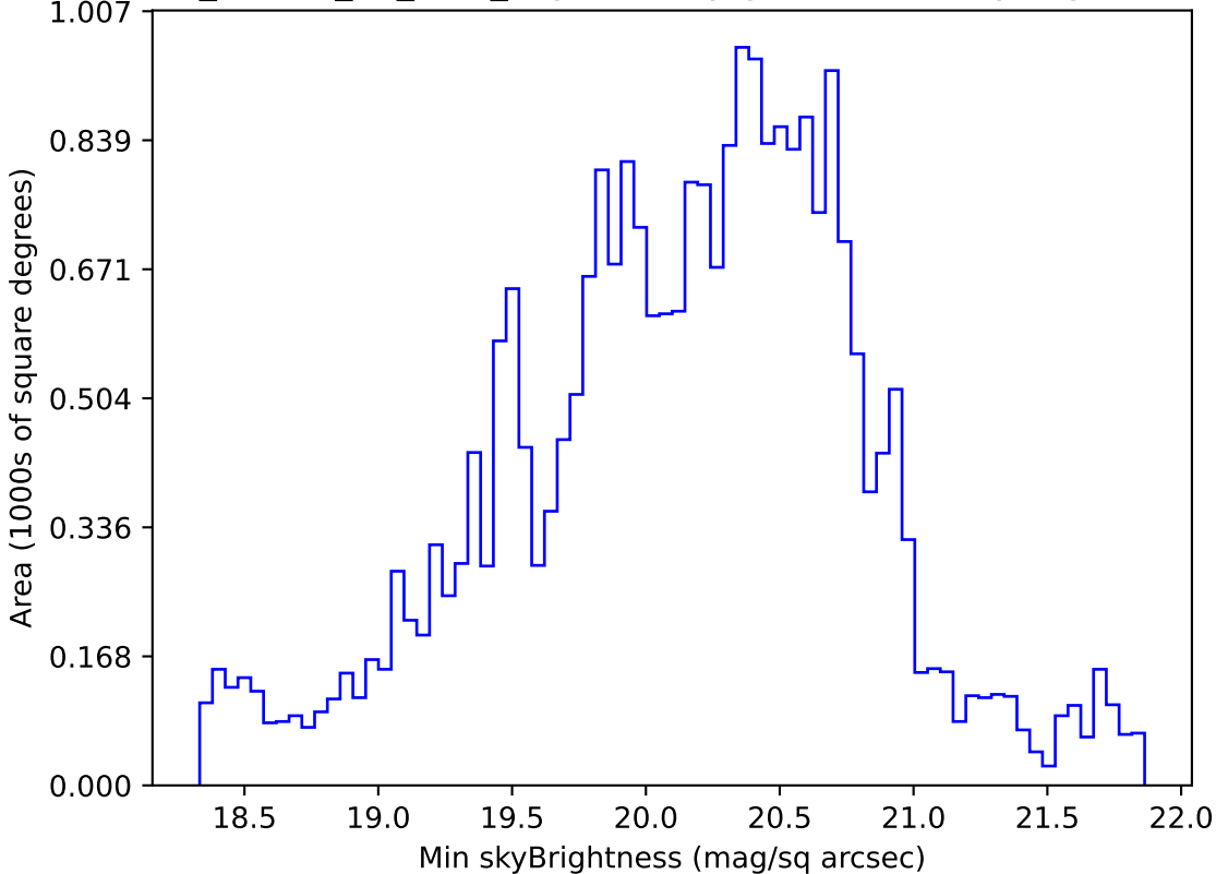
ddf_loaded_fl2_v3.4_10yrs All sky g band: Min skyBrightness
