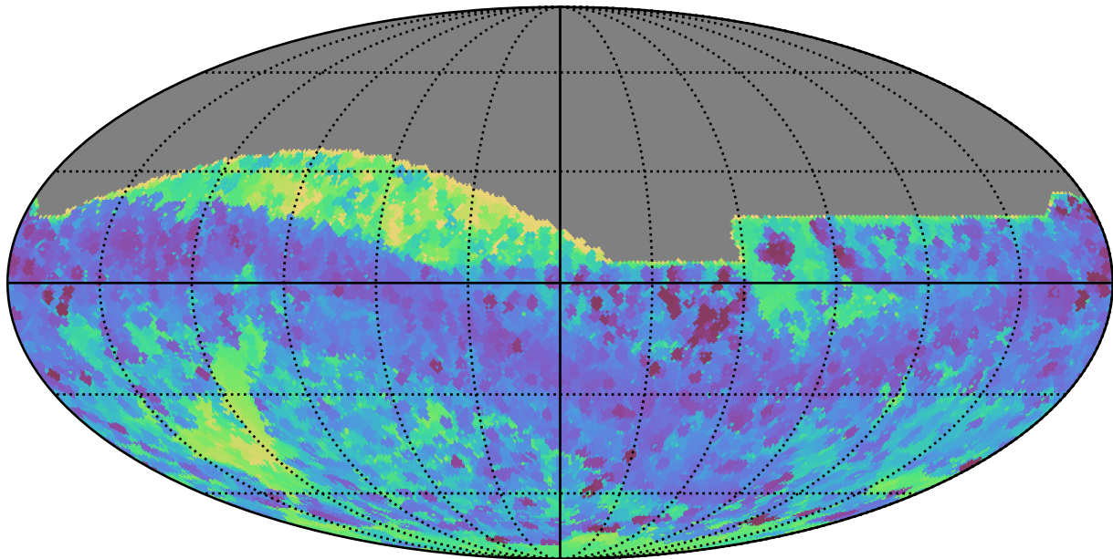
ddf_loaded_fl2_v3.4_10yrs All sky all bands: Min skyBrightness
