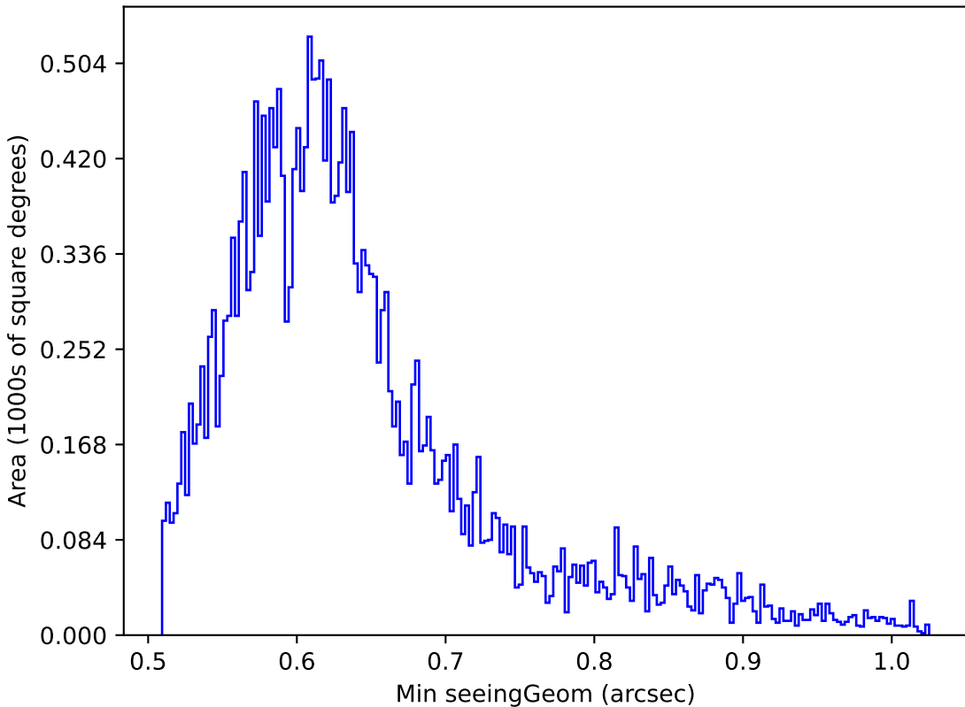
ddf_loaded_fl2_v3.4_10yrs Yr 1 z band: Min seeingGeom
