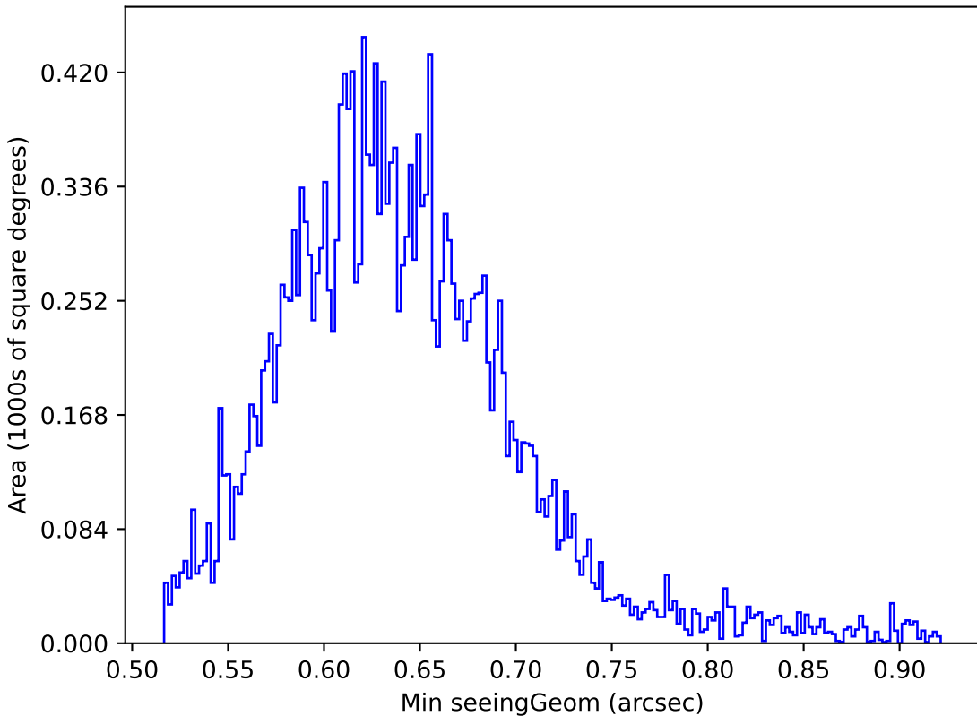
ddf_loaded_fl2_v3.4_10yrs Yr 1 y band: Min seeingGeom
