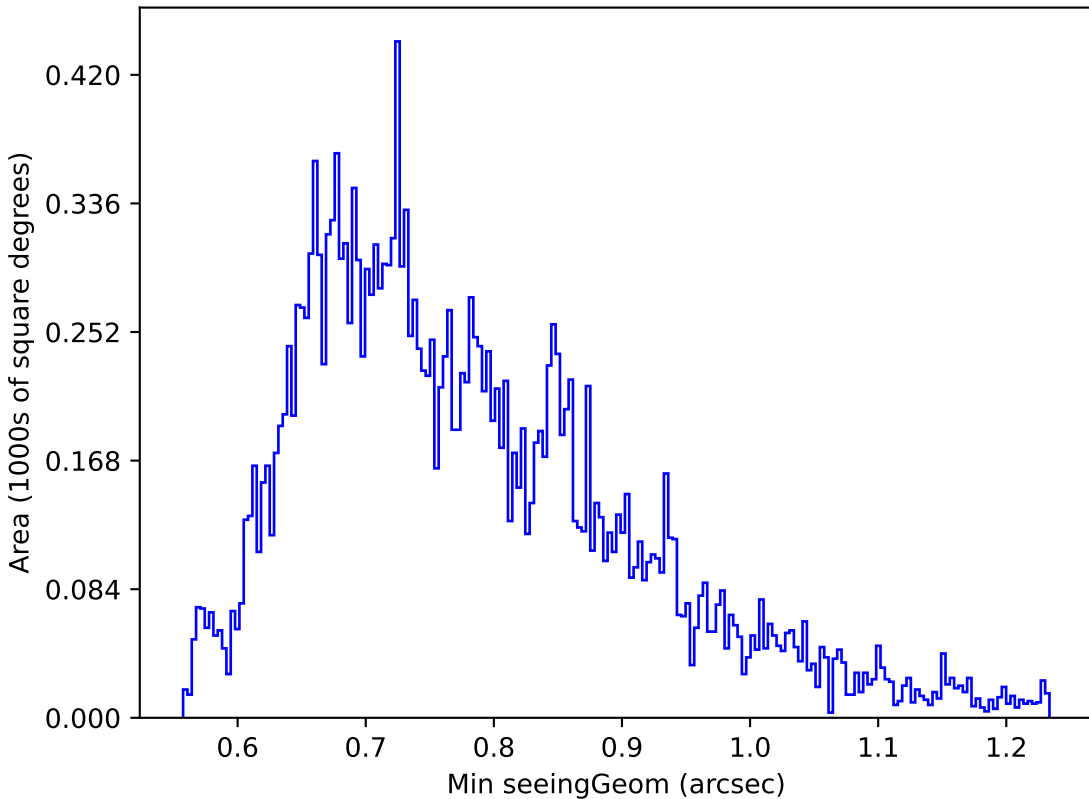
ddf_loaded_fl2_v3.4_10yrs Yr 1 u band: Min seeingGeom
