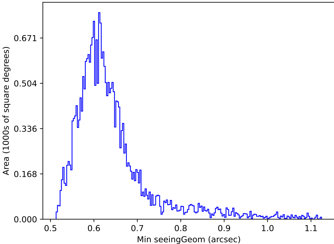
ddf_loaded_fl2_v3.4_10yrs Yr 1 r band: Min seeingGeom
