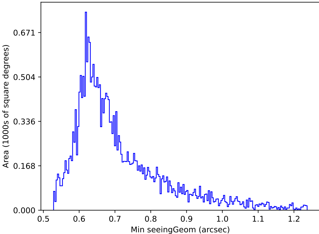
ddf_loaded_fl2_v3.4_10yrs Yr 1 g band: Min seeingGeom
