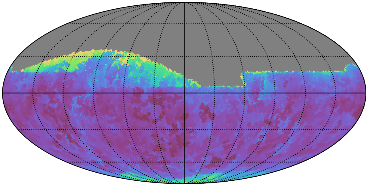
ddf_loaded_fl2_v3.4_10yrs Yr 1 all bands: Min seeingGeom
