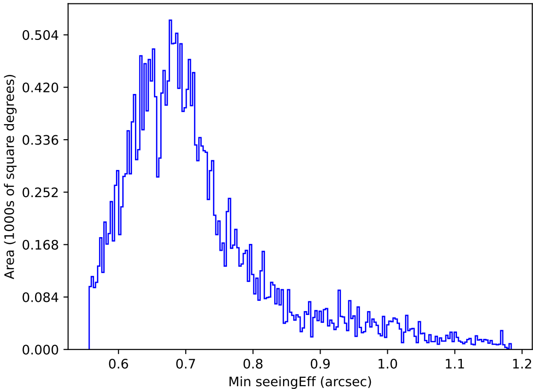
ddf_loaded_fl2_v3.4_10yrs Yr 1 z band: Min seeingEff
