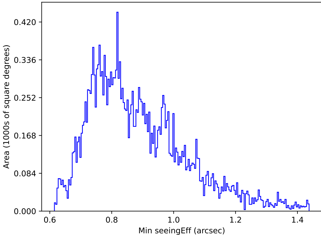
ddf_loaded_fl2_v3.4_10yrs Yr 1 u band: Min seeingEff
