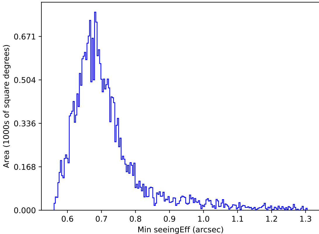
ddf_loaded_fl2_v3.4_10yrs Yr 1 r band: Min seeingEff
