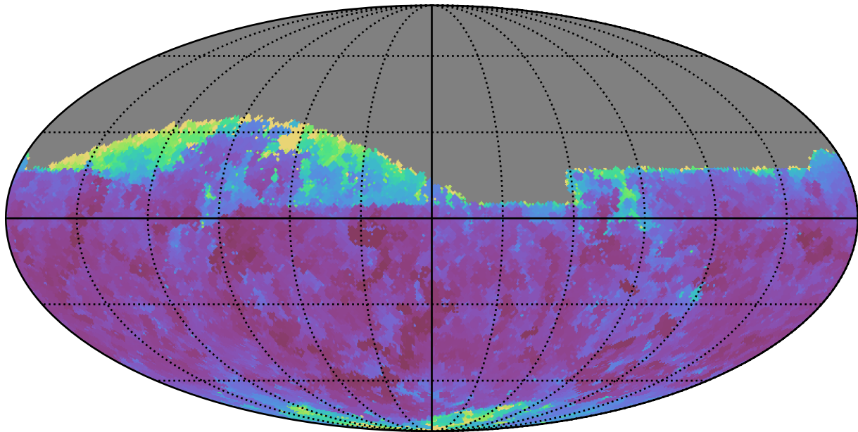
ddf_loaded_fl2_v3.4_10yrs Yr 1 i band: Min seeingEff
