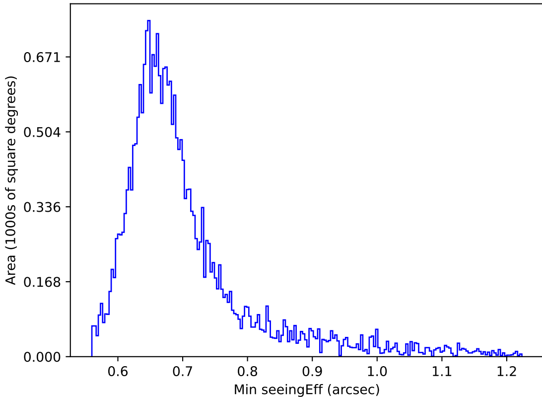
ddf_loaded_fl2_v3.4_10yrs Yr 1 i band: Min seeingEff
