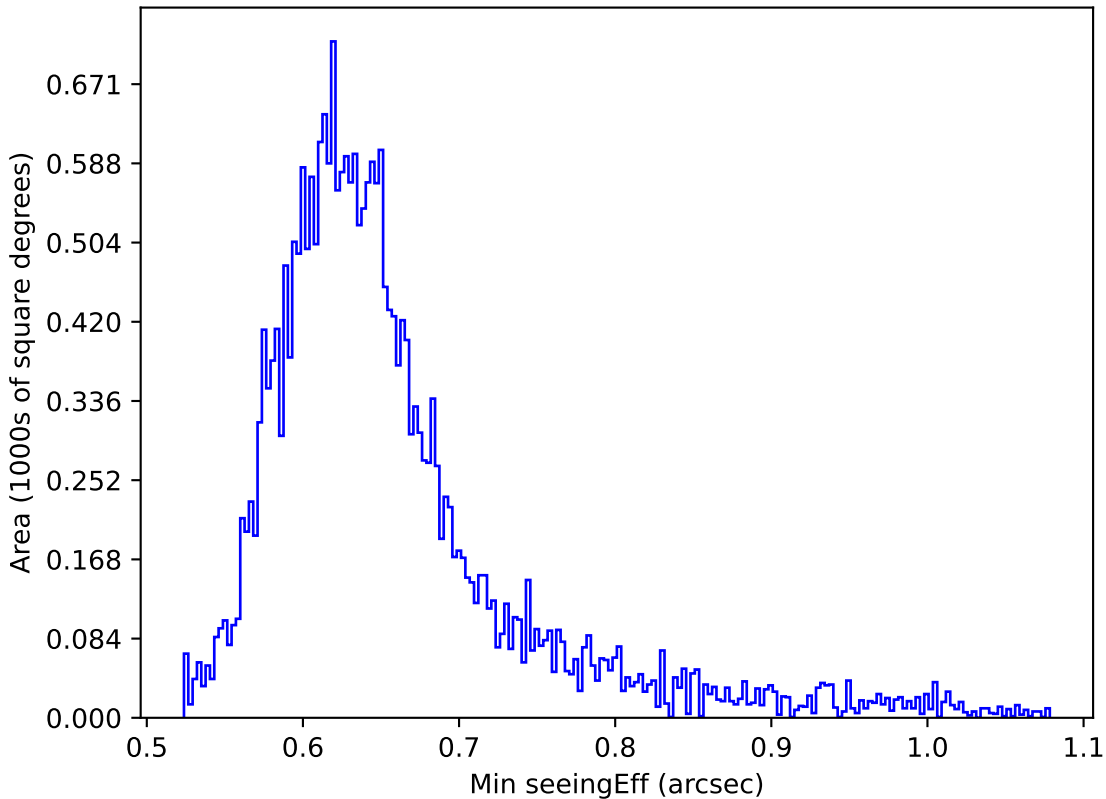
ddf_loaded_fl2_v3.4_10yrs Yr 1 all bands: Min seeingEff
