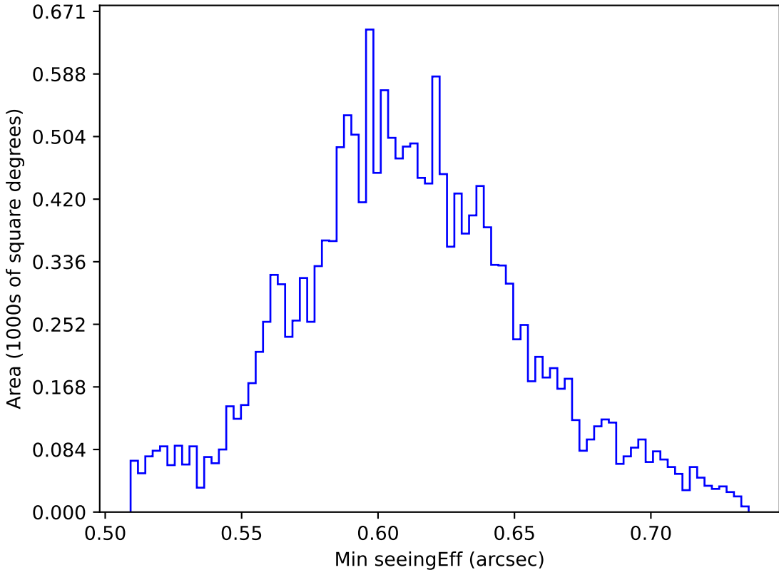
ddf_loaded_fl2_v3.4_10yrs WFD z band: Min seeingEff
