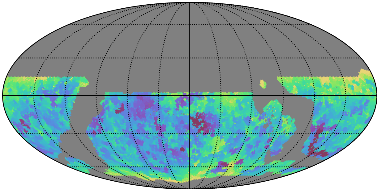
ddf_loaded_fl2_v3.4_10yrs WFD y band: Min seeingEff
