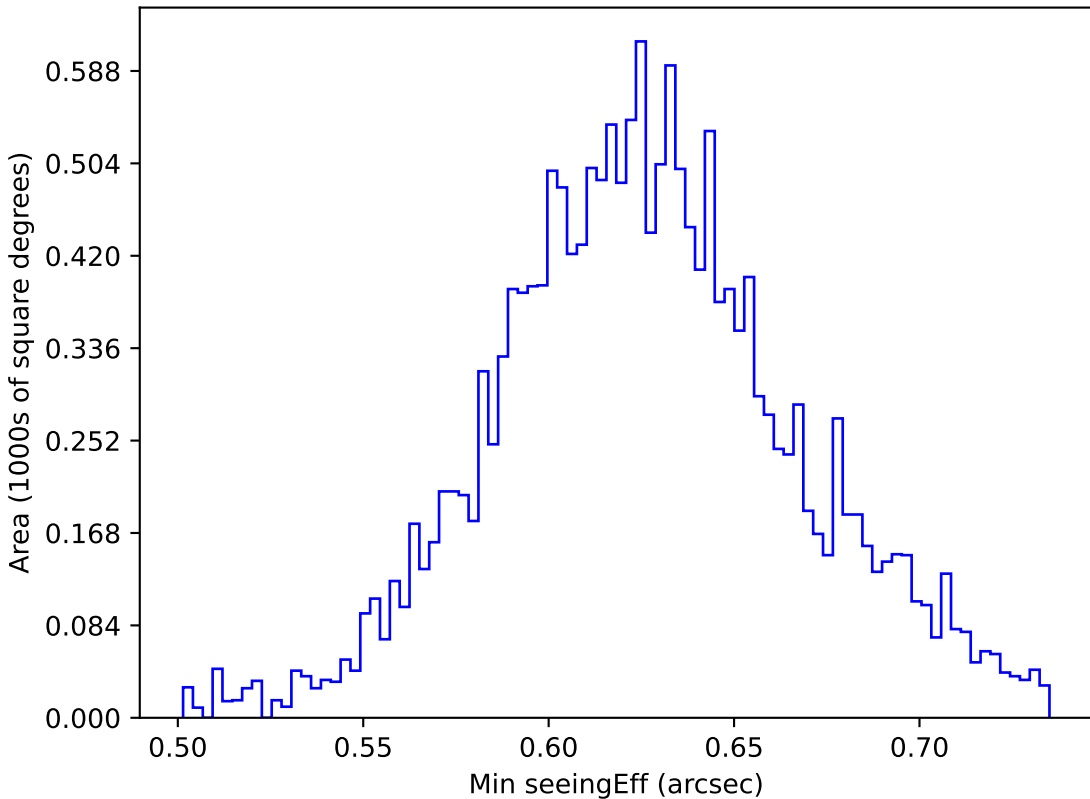
ddf_loaded_fl2_v3.4_10yrs WFD y band: Min seeingEff
