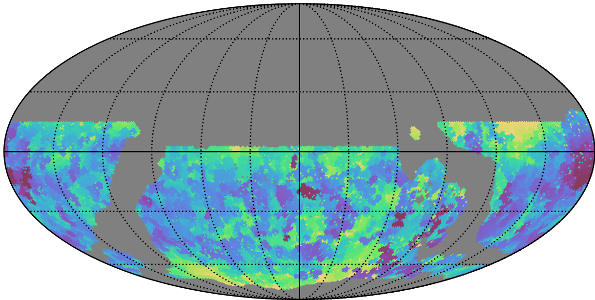
ddf_loaded_fl2_v3.4_10yrs WFD u band: Min seeingEff
