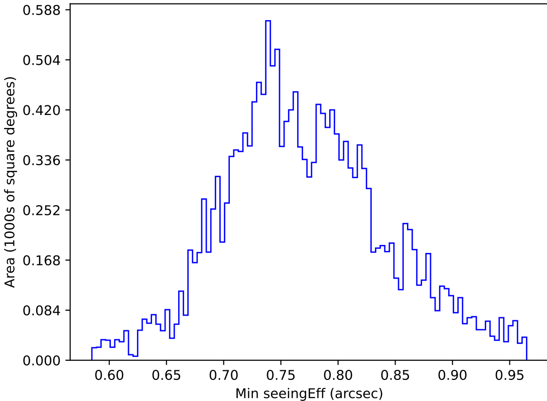
ddf_loaded_fl2_v3.4_10yrs WFD u band: Min seeingEff
