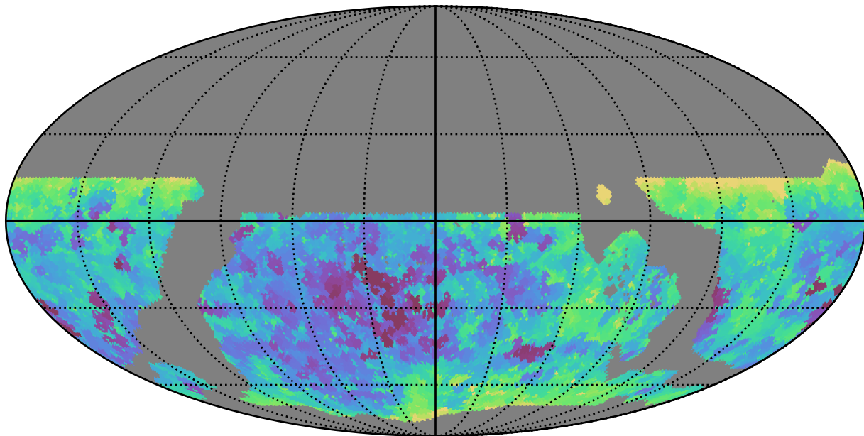
ddf_loaded_fl2_v3.4_10yrs WFD r band: Min seeingEff
