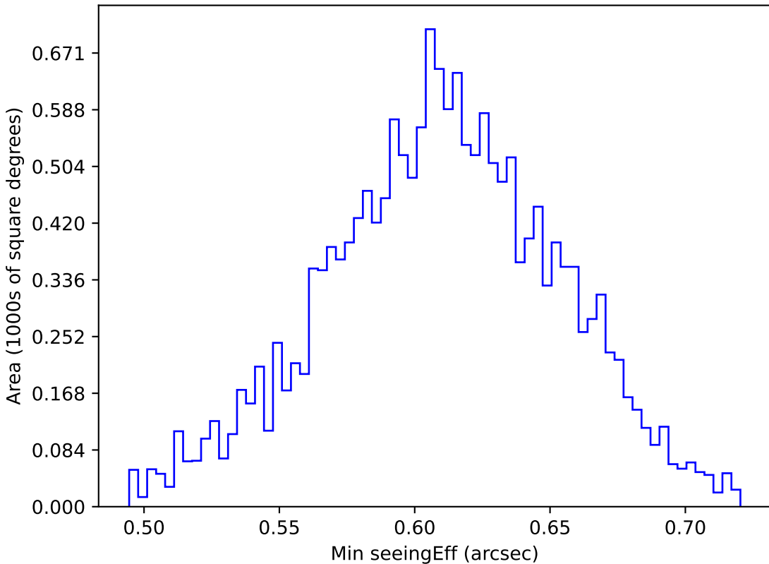
ddf_loaded_fl2_v3.4_10yrs WFD r band: Min seeingEff
