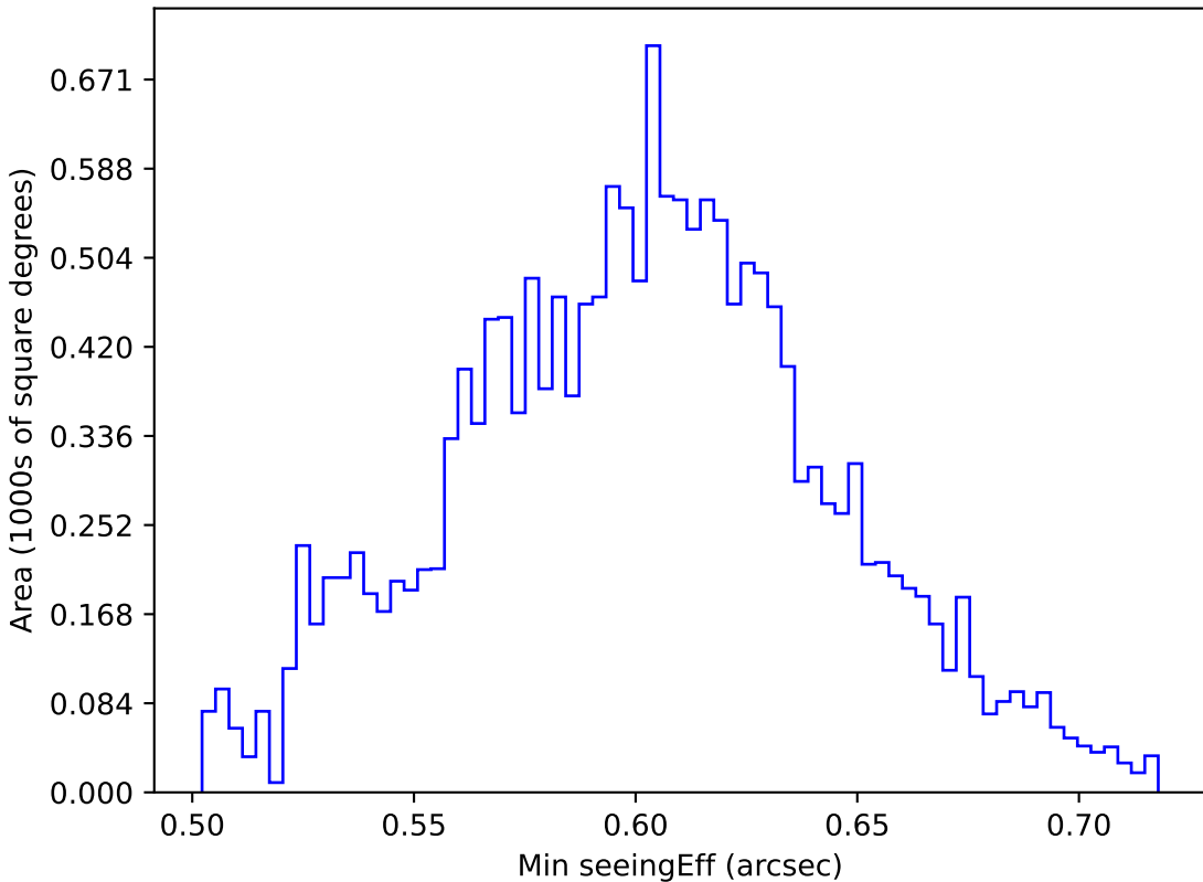
ddf_loaded_fl2_v3.4_10yrs WFD i band: Min seeingEff
