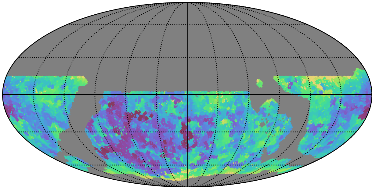
ddf_loaded_fl2_v3.4_10yrs WFD g band: Min seeingEff
