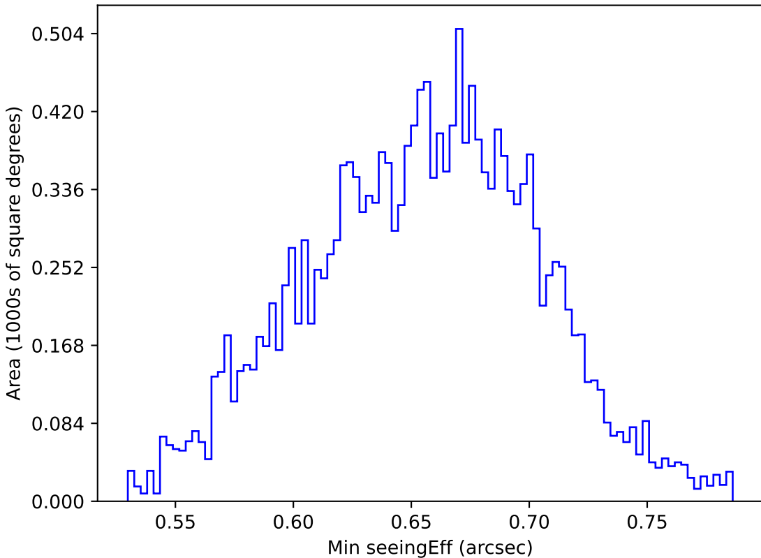
ddf_loaded_fl2_v3.4_10yrs WFD g band: Min seeingEff
