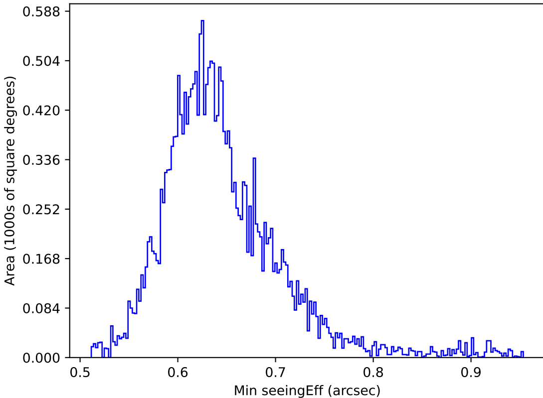
ddf_loaded_fl2_v3.4_10yrs All sky y band: Min seeingEff
