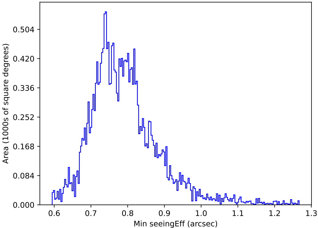
ddf_loaded_fl2_v3.4_10yrs All sky u band: Min seeingEff
