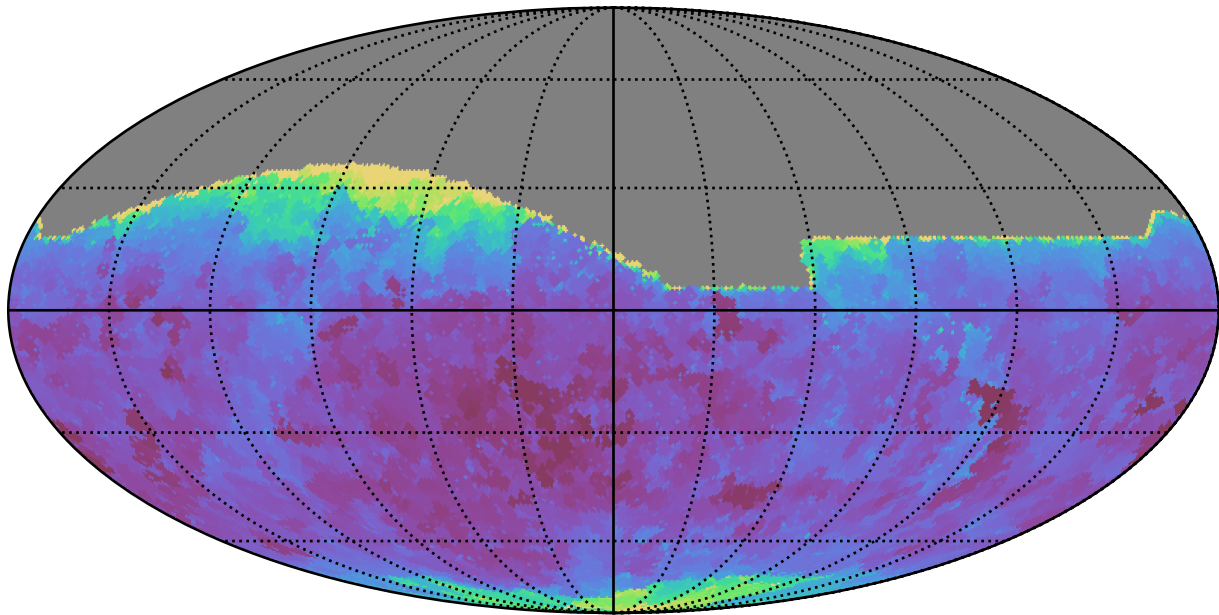
ddf_loaded_fl2_v3.4_10yrs All sky r band: Min seeingEff
