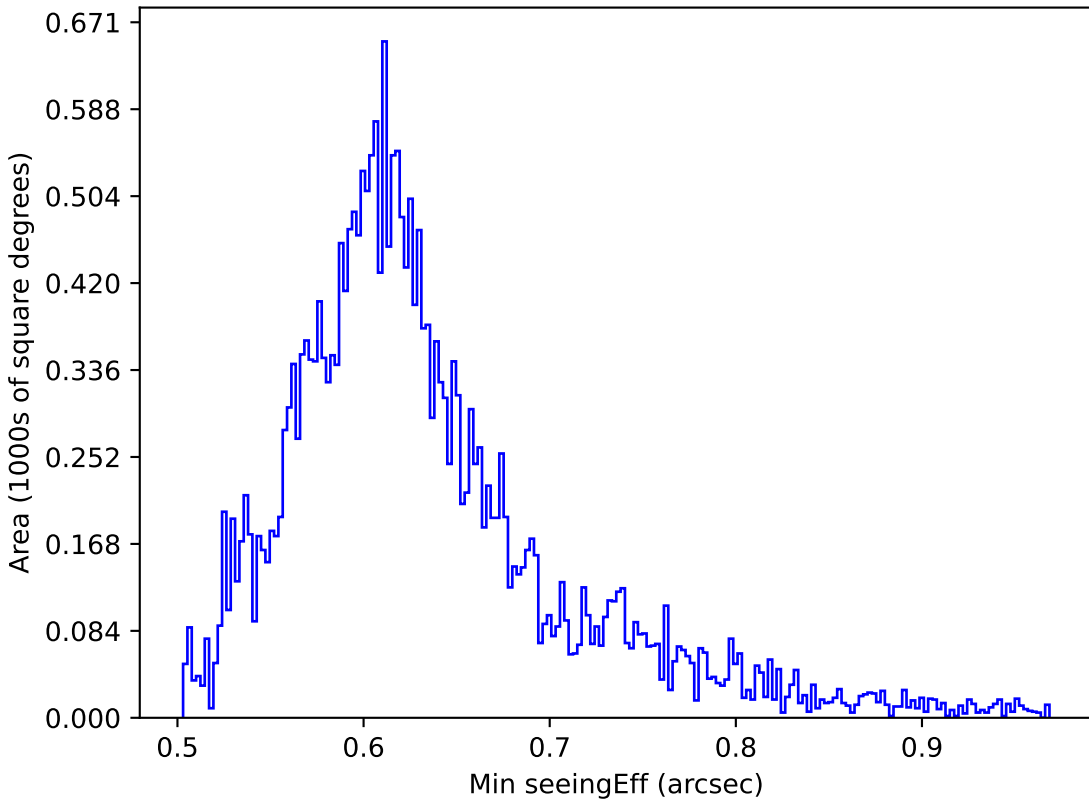
ddf_loaded_fl2_v3.4_10yrs All sky i band: Min seeingEff
