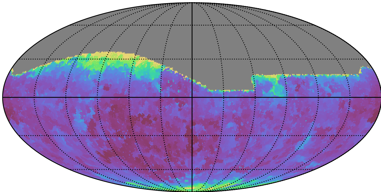
ddf_loaded_fl2_v3.4_10yrs All sky g band: Min seeingEff
