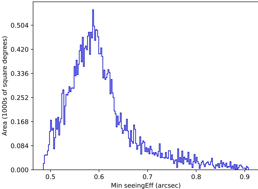
ddf_loaded_fl2_v3.4_10yrs All sky all bands: Min seeingEff
