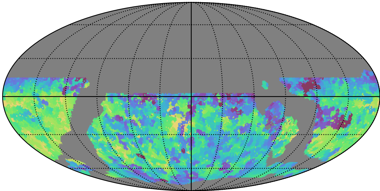
ddf_loaded_fl2_v3.4_10yrs WFD u band: Min saturation_mag
