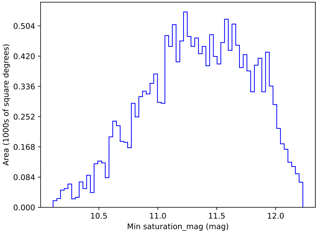
ddf_loaded_fl2_v3.4_10yrs WFD u band: Min saturation_mag
