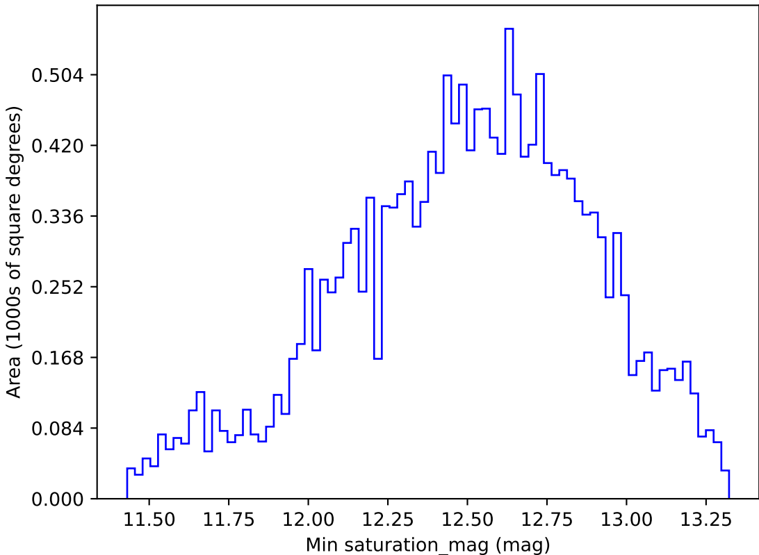
ddf_loaded_fl2_v3.4_10yrs WFD r band: Min saturation_mag
