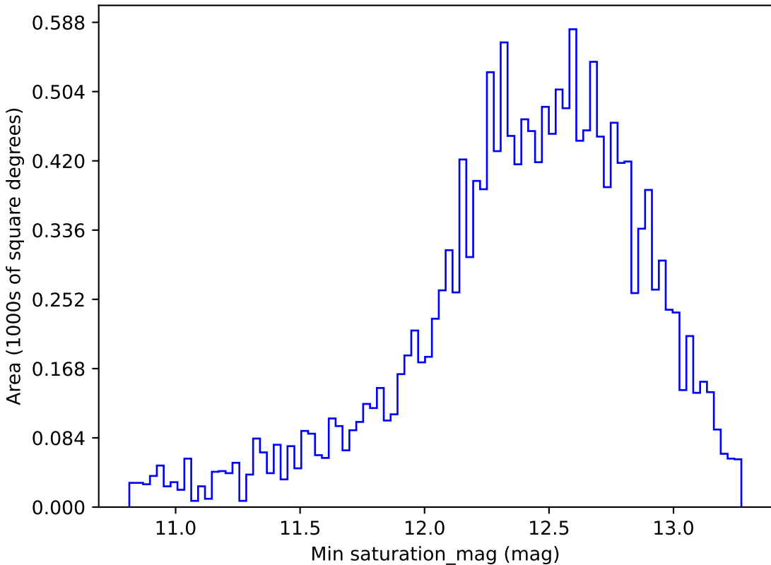
ddf_loaded_fl2_v3.4_10yrs WFD i band: Min saturation_mag
