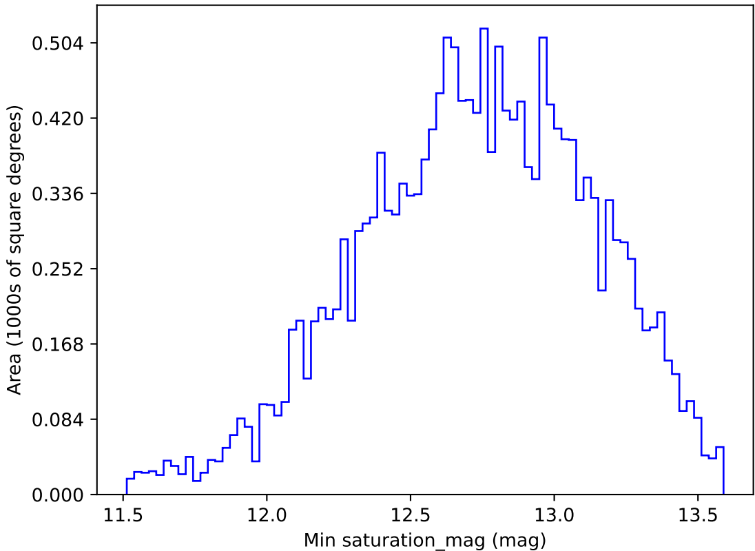
ddf_loaded_fl2_v3.4_10yrs WFD g band: Min saturation_mag
