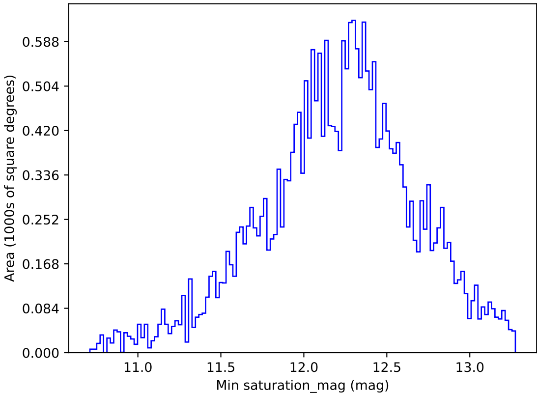
ddf_loaded_fl2_v3.4_10yrs All sky z band: Min saturation_mag
