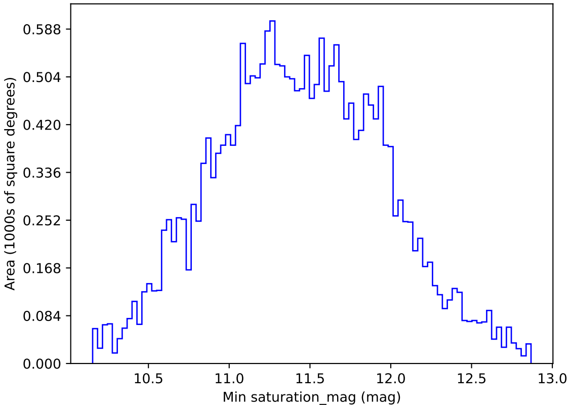
ddf_loaded_fl2_v3.4_10yrs All sky u band: Min saturation_mag
