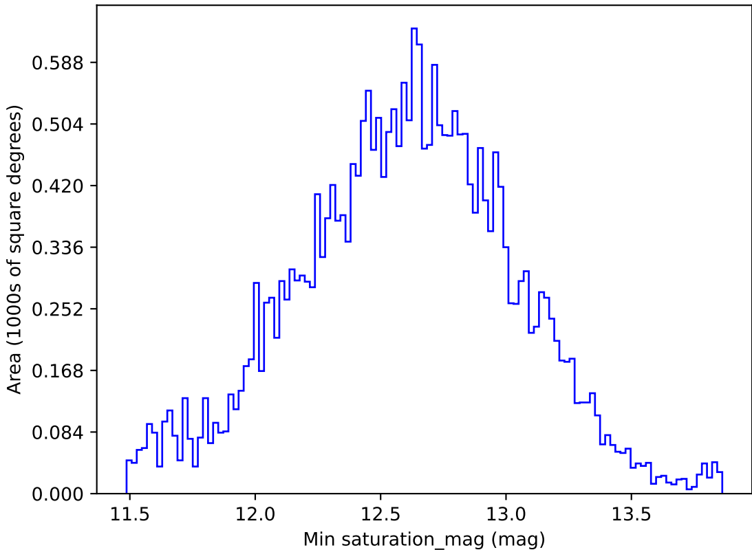
ddf_loaded_fl2_v3.4_10yrs All sky r band: Min saturation_mag
