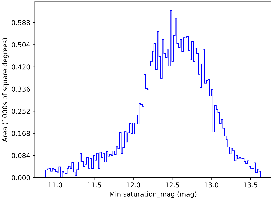
ddf_loaded_fl2_v3.4_10yrs All sky i band: Min saturation_mag
