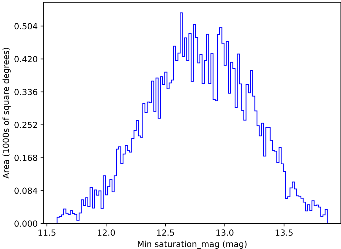
ddf_loaded_fl2_v3.4_10yrs All sky g band: Min saturation_mag
