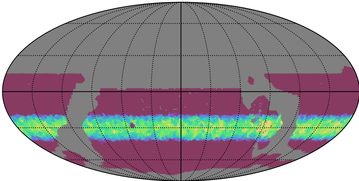
ddf_loaded_fl2_v3.4_10yrs WFD y band: Min normairmass
