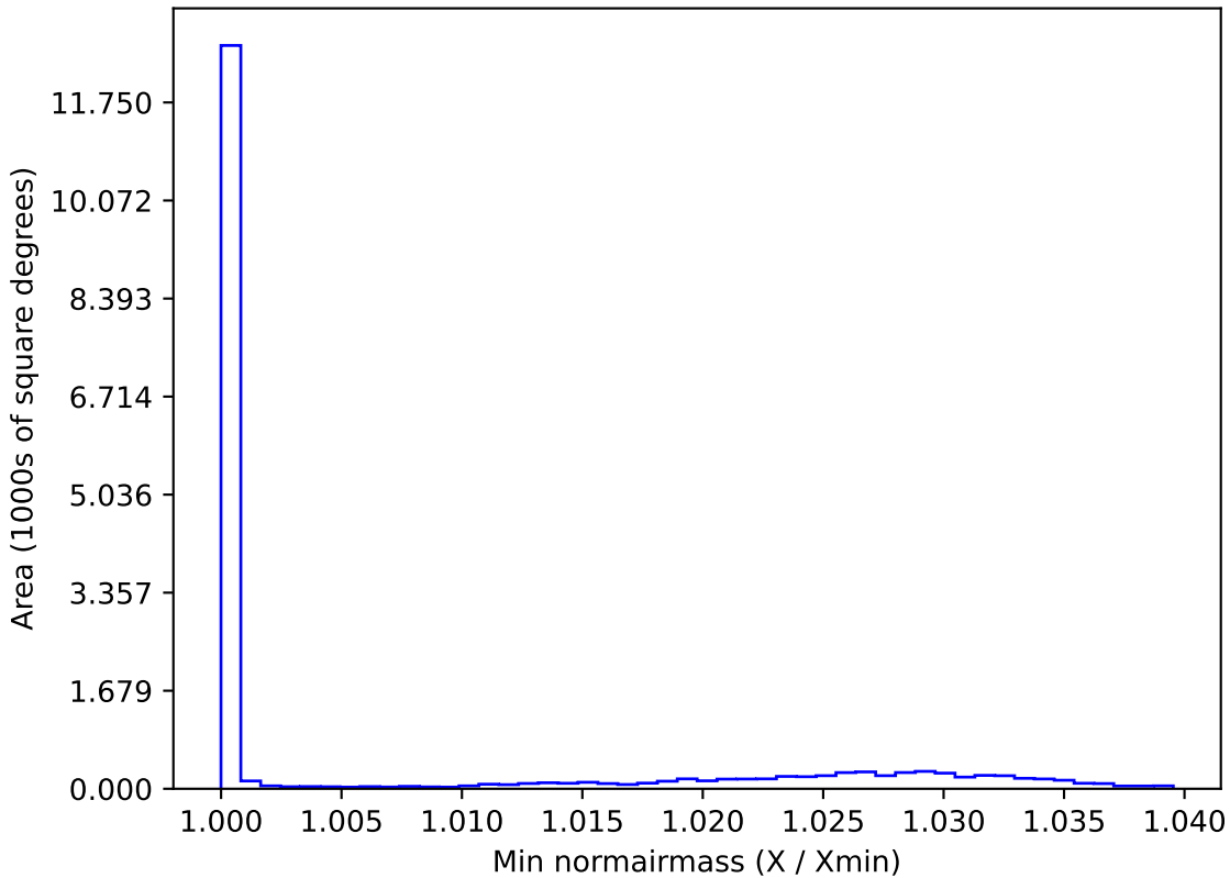
ddf_loaded_fl2_v3.4_10yrs WFD y band: Min normairmass
