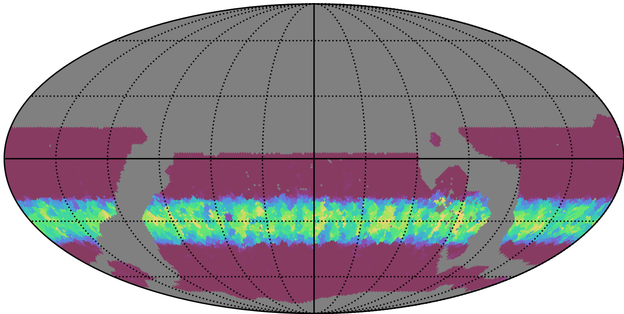
ddf_loaded_fl2_v3.4_10yrs WFD u band: Min normairmass
