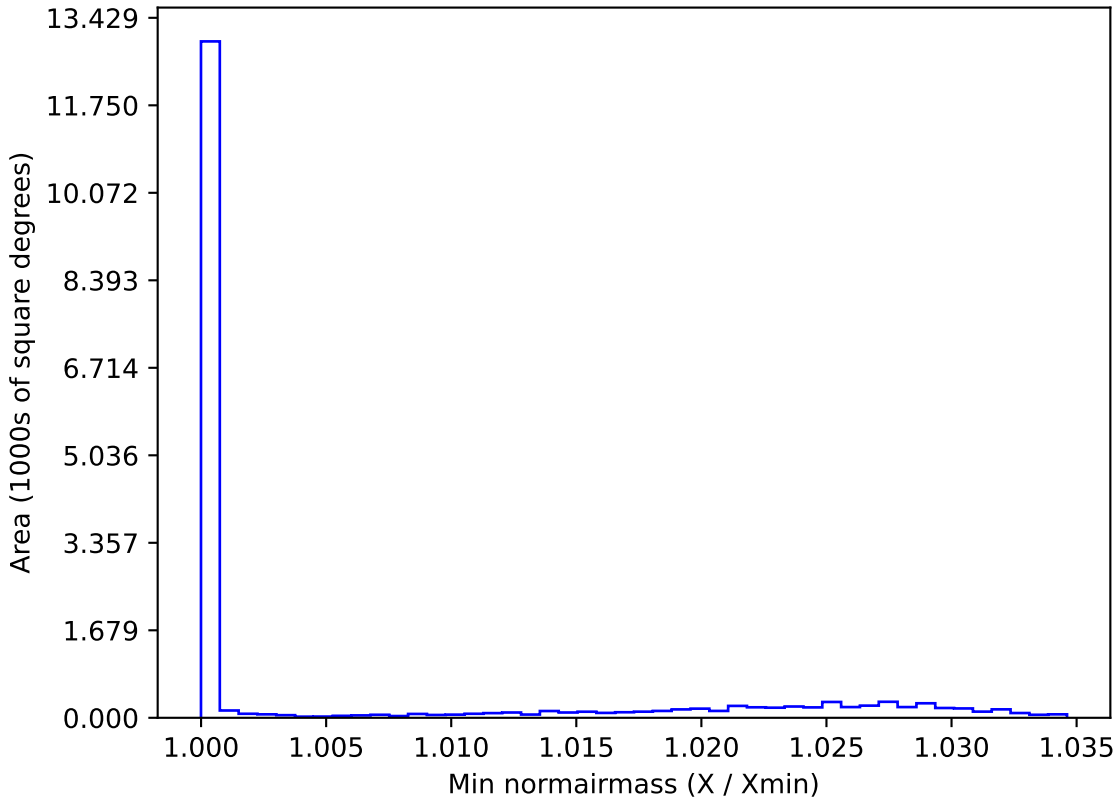
ddf_loaded_fl2_v3.4_10yrs WFD i band: Min normairmass
