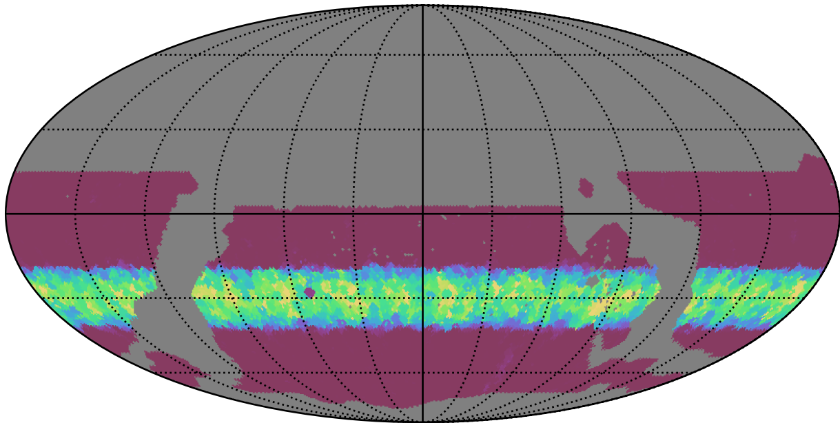
ddf_loaded_fl2_v3.4_10yrs WFD g band: Min normairmass
