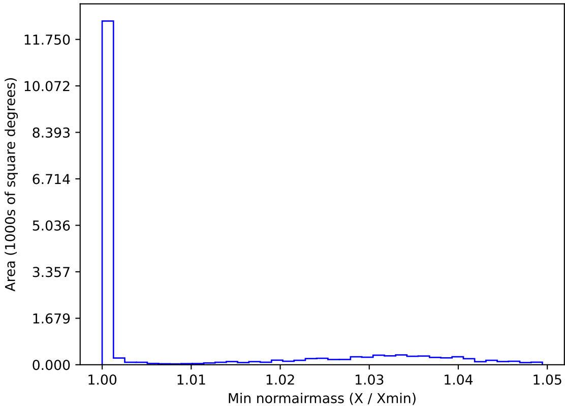
ddf_loaded_fl2_v3.4_10yrs WFD g band: Min normairmass
