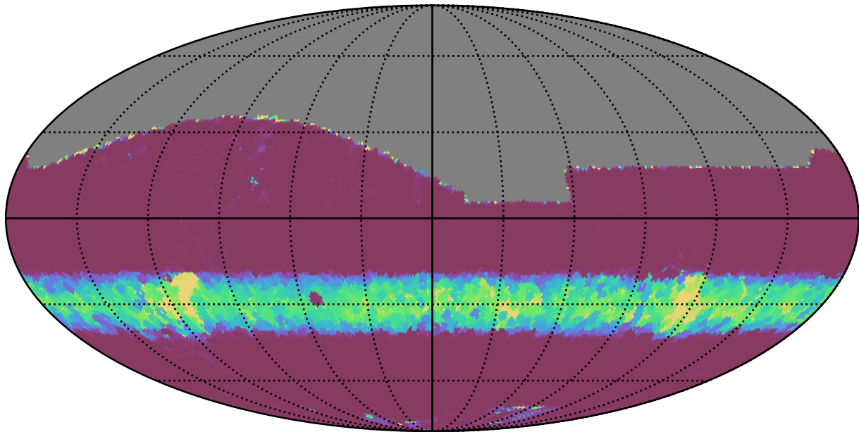
ddf_loaded_fl2_v3.4_10yrs All sky z band: Min normairmass
