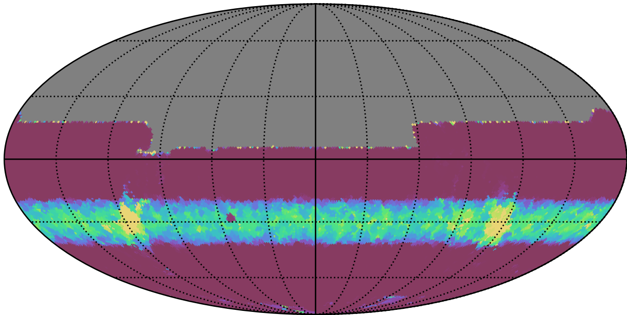
ddf_loaded_fl2_v3.4_10yrs All sky y band: Min normairmass
