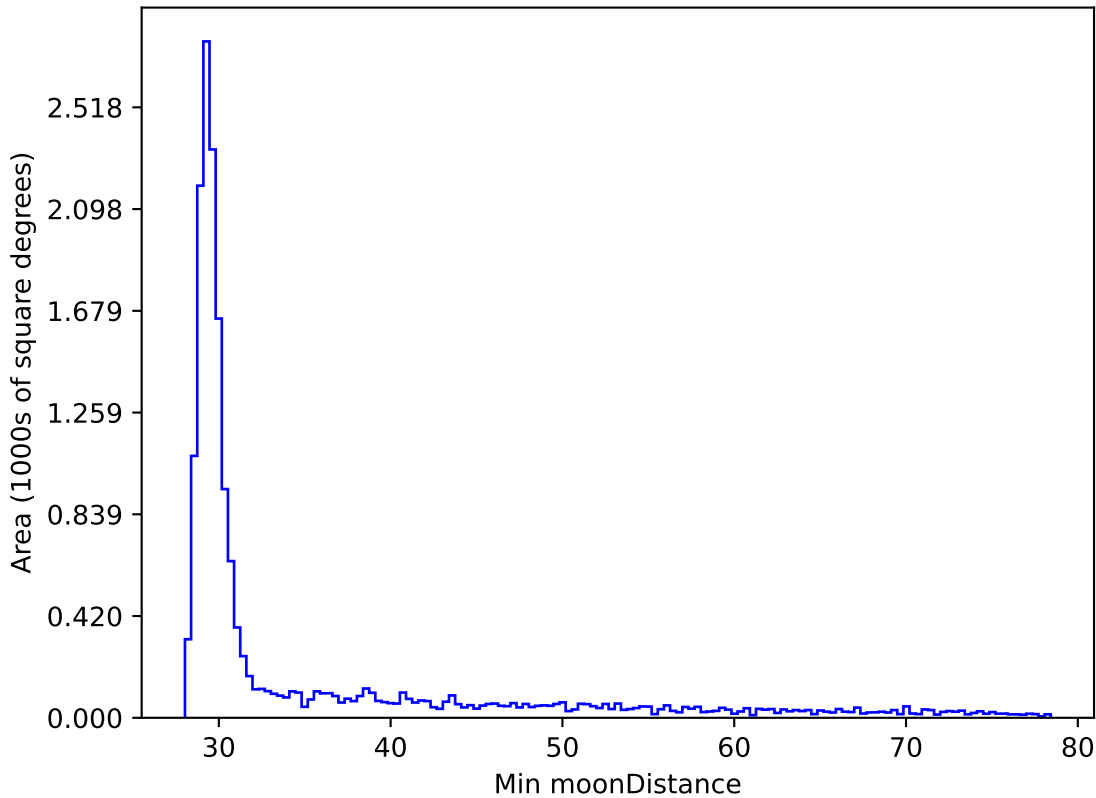
ddf_loaded_fl2_v3.4_10yrs WFD y band: Min moonDistance
