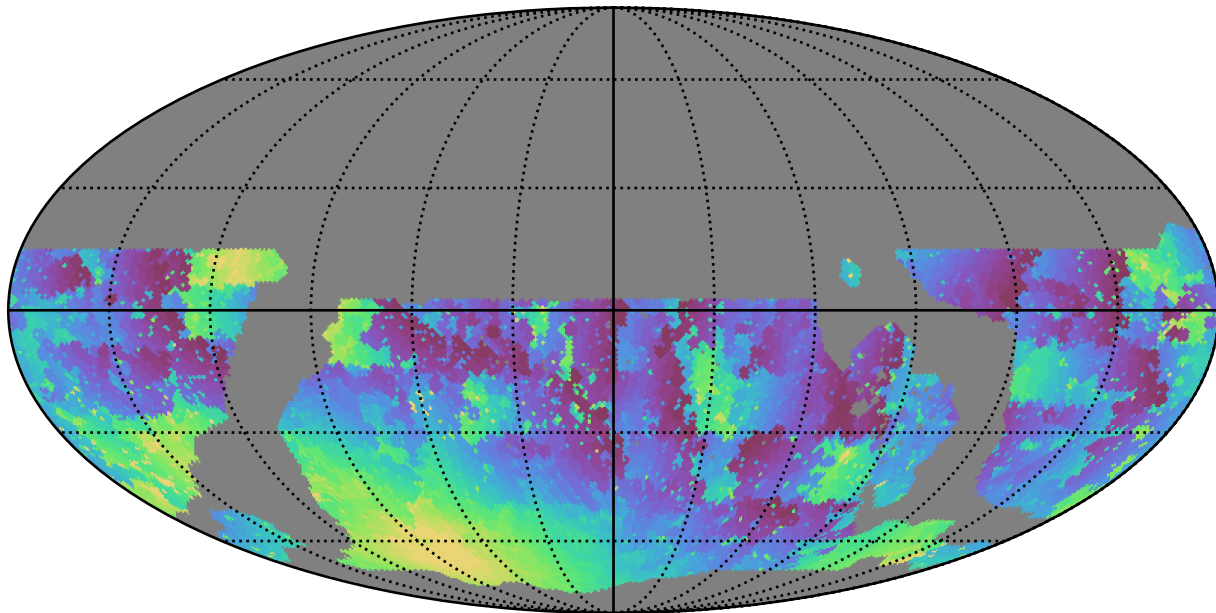
ddf_loaded_fl2_v3.4_10yrs WFD u band: Min moonDistance
